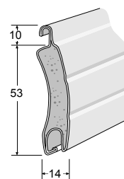
Lamellprofil Standard Safe Aluminium
